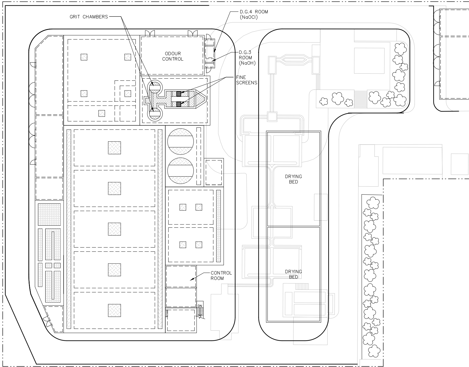
Figure 2-4b General Layout for Proposed Peng Chau STW Upgrade - Roof Floor Plan
